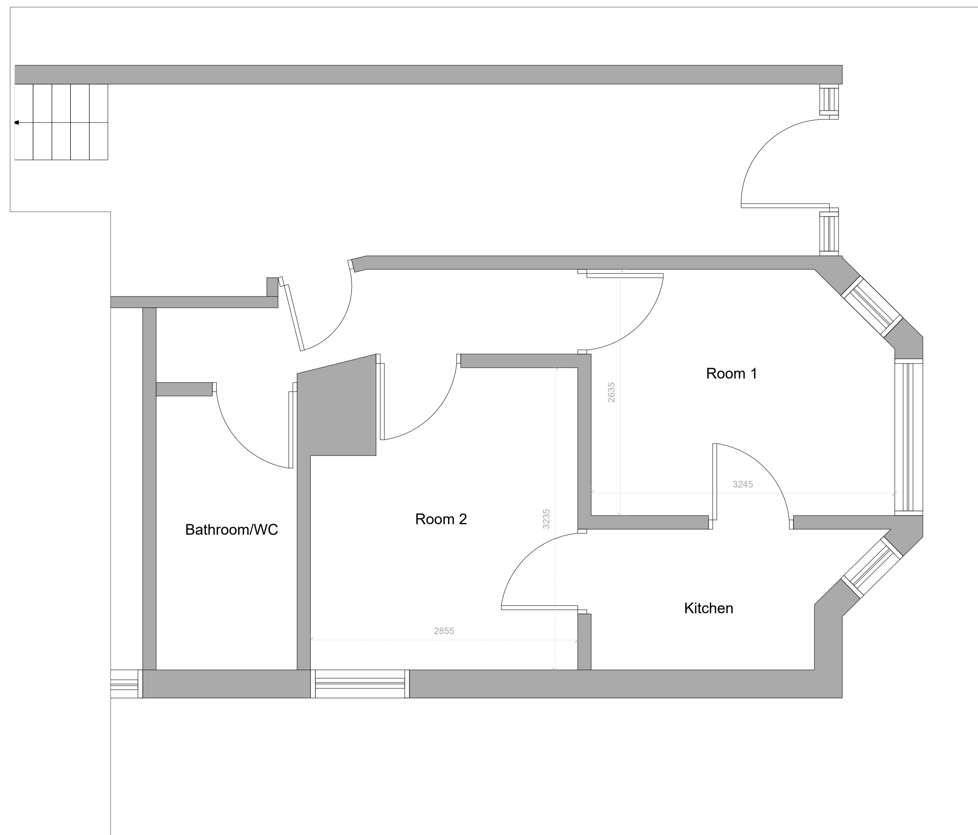
FIRST FLOOR
